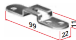
art. 2200 Staffa incassabile Embedded bracket
