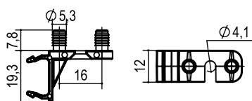
铝型材卡扣 P.A549.16.53
