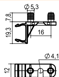
铝型材卡扣 P.A549.16.53
